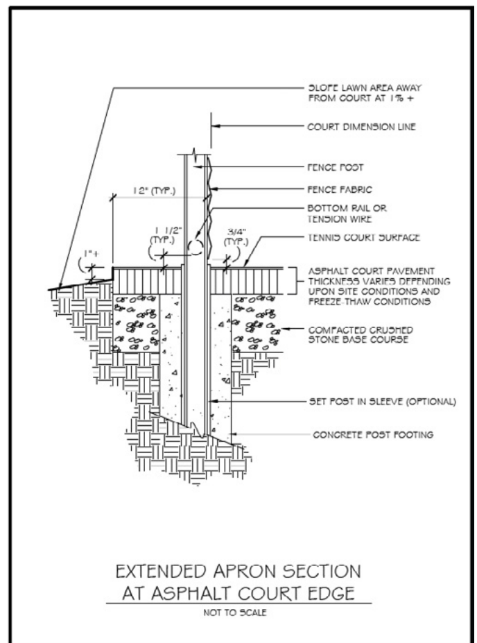
Figure 12. Extended Apron Section at Asphalt Court Edge.
