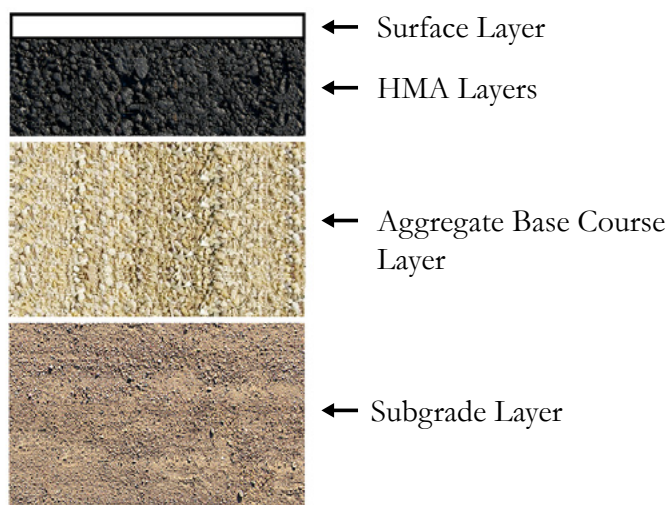
Figure 10. Asphalt Game Court Layers
