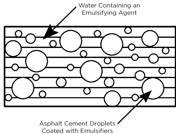
Figure 3.1. Emulsified Asphalt
