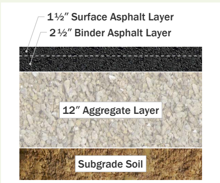
Figure 2 Completed standard 4-inch asphalt pavement
